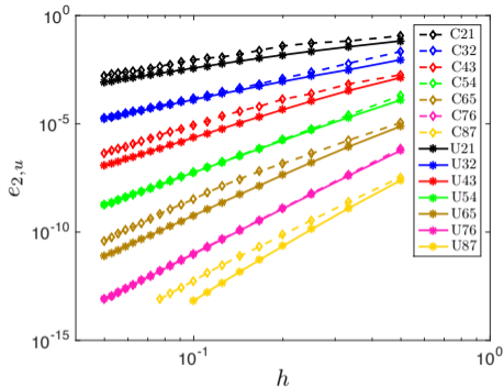
Figure 4: Harmonic Vibrations of the unit square. Errors at the final time for the harmonic vibrations of the traction free unit square. To the left q_u = q_v + 1 = 2, \dots, 8 with central and upwind flux. To the right q_u = q_v = 2, \dots, 8 with central and upwind flux.
